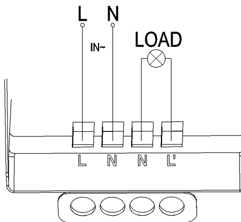
Connection-wire diagram
